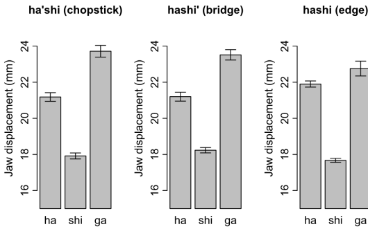
Figure 2 The Jaw displacement patterns of the accentually minimal triplet by Speaker J06. Y-axis represents the degree of jaw displacement (mm). The error bars represent standard errors. To show observed jaw displacement patterns, different figures in this paper use different y-axis scale.
